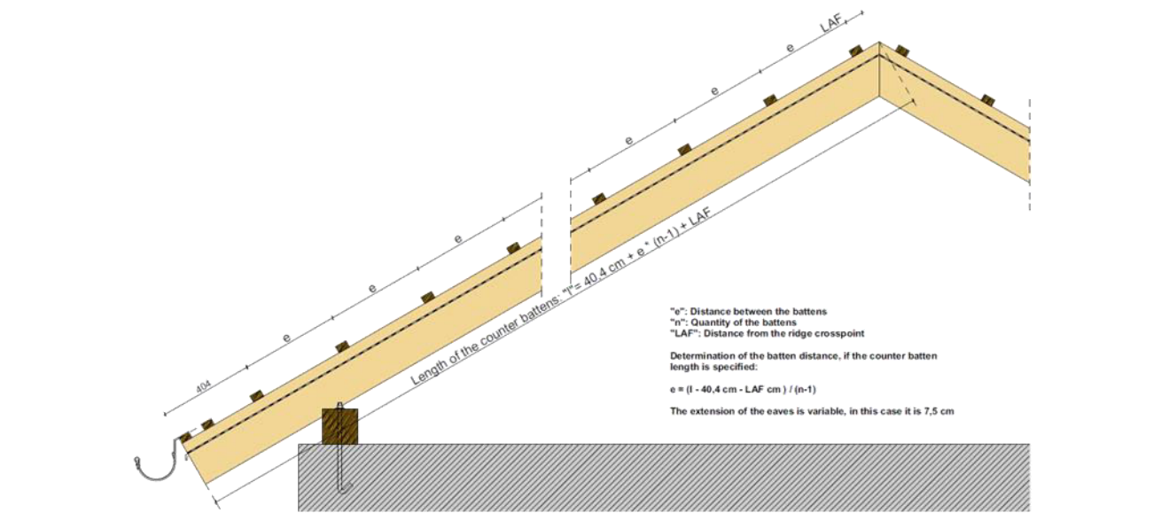
Roof batten alignment for “SIMPLA” clay roof tile
