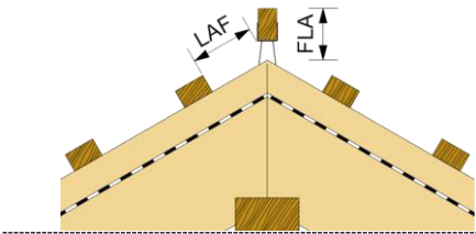
LAF: distance of the upper batten FLA: height of the ridge batten
