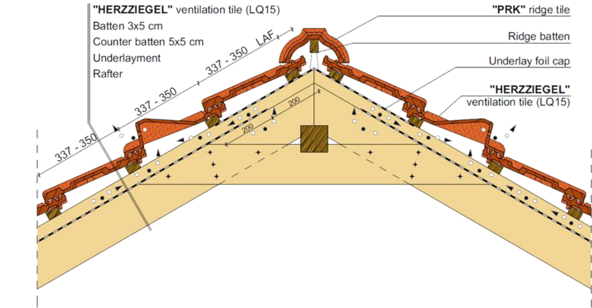
Ridge detail, with ventilation tile
