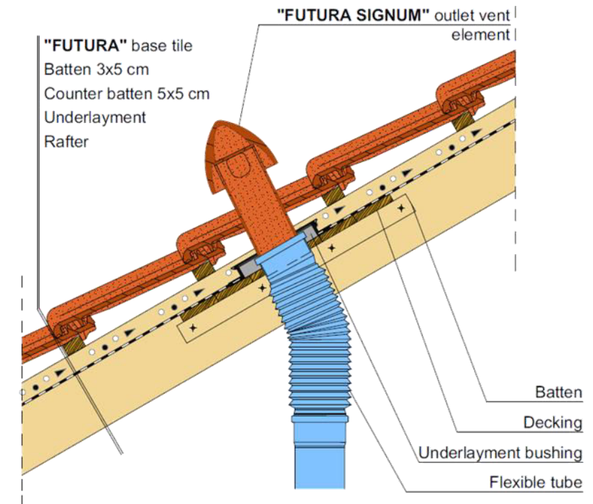
Clay ventilation outlet tile
