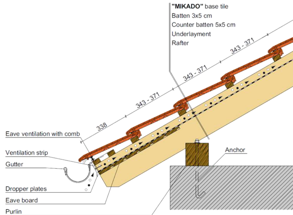
Eave detail
