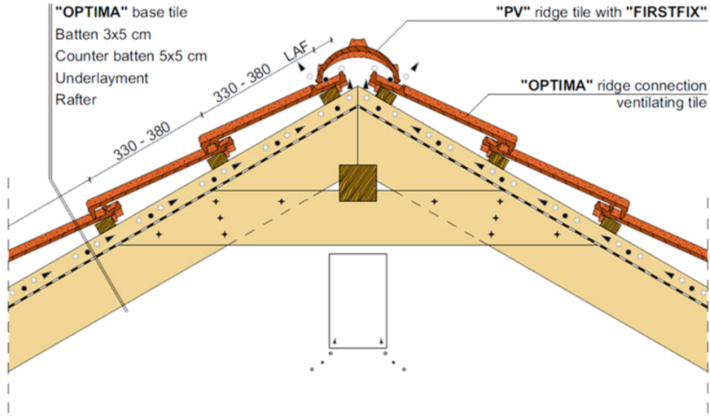
Ridge detail, with ridge connection ventilation tile
