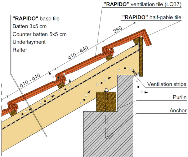
Shed ridge detail, with shad roof tile
