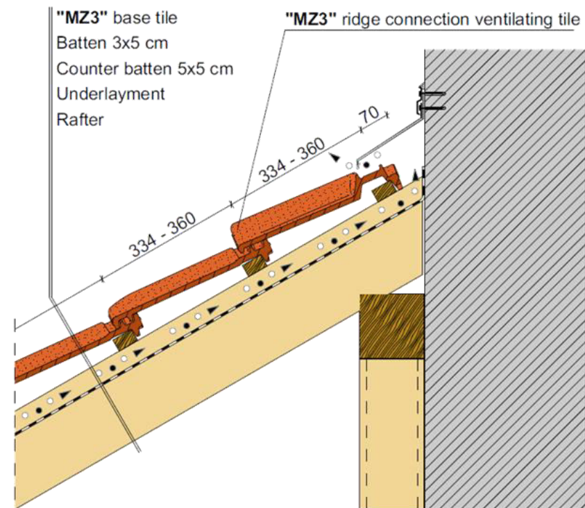
Wall connection detail
