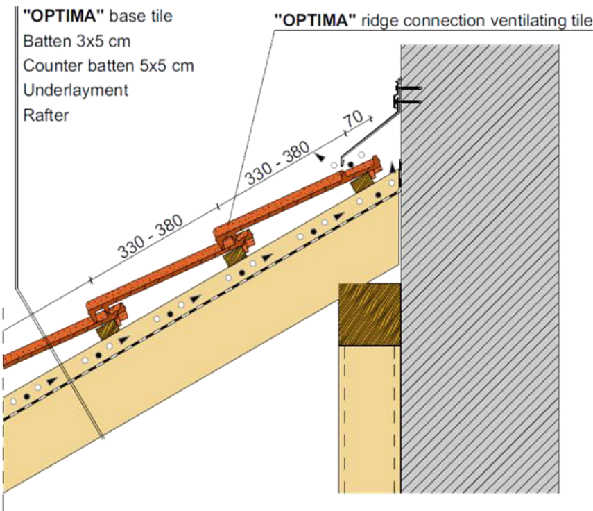
Wall connection detail
