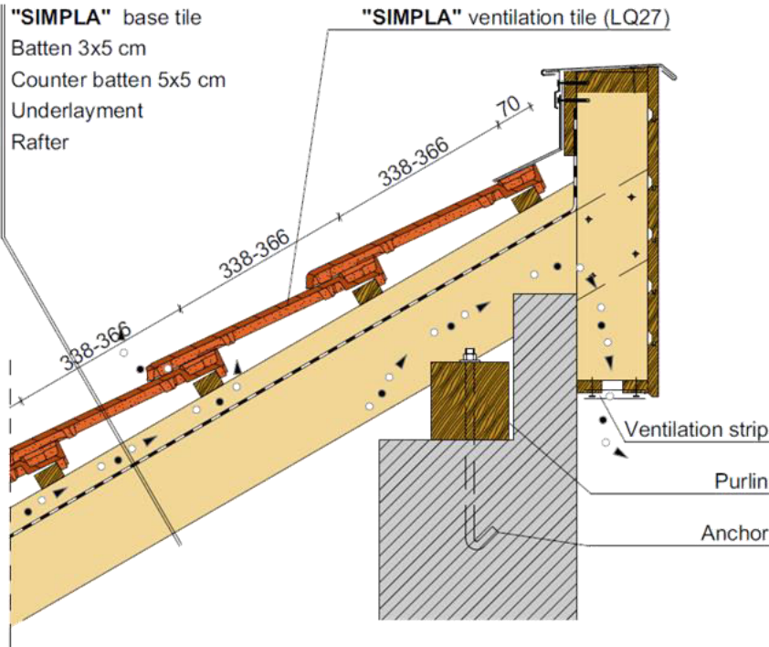
Shed ridge detail, with shad roof tile
