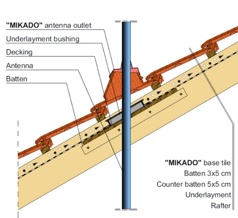
Clay antenna outlet tile
