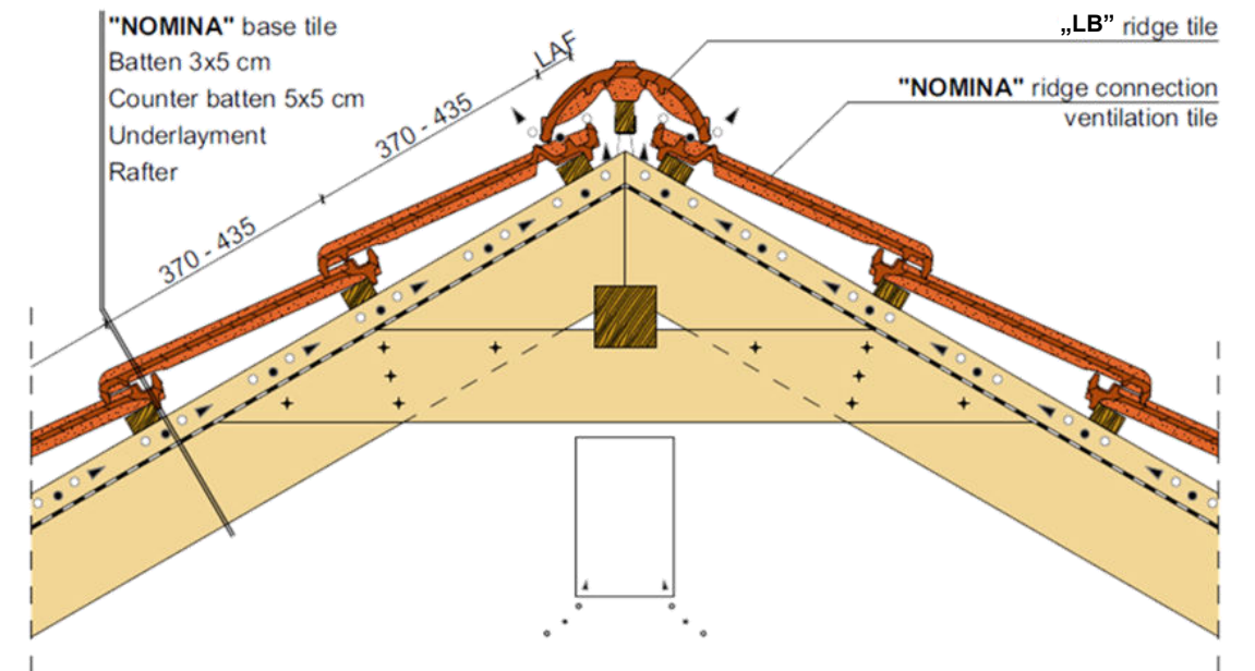
Ridge detail, with ridge connection ventilation tile
