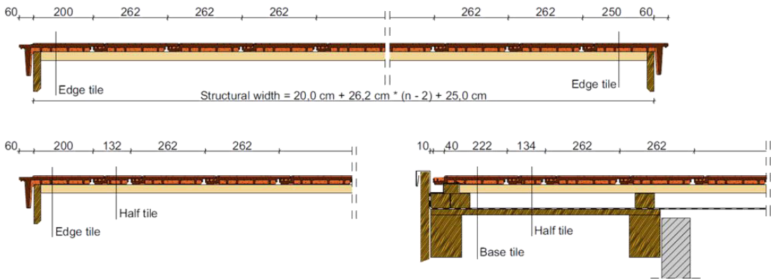
Structural width between the verge boards
