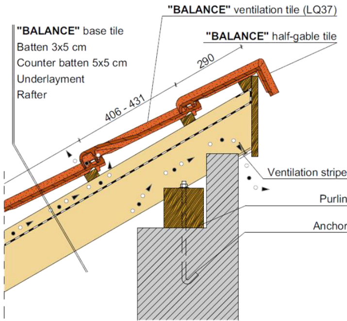
Shed ridge detail, with shad roof tile
