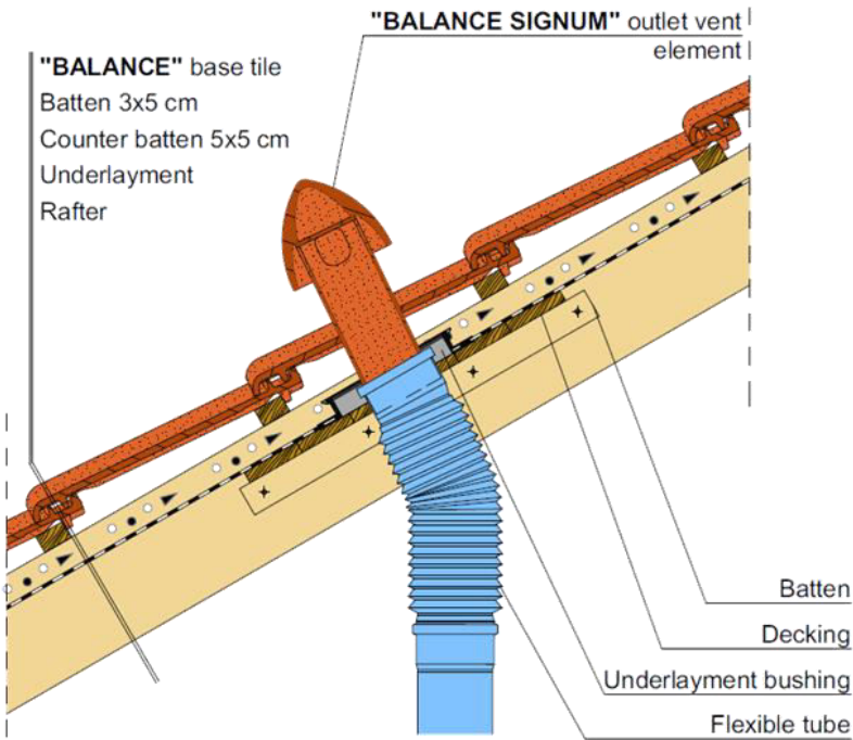
Clay ventilation outlet tile
