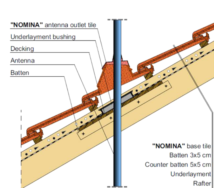
Clay antenna outlet tile
