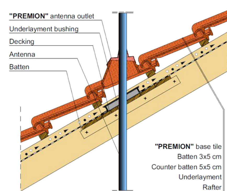
Clay antenna outlet tile
