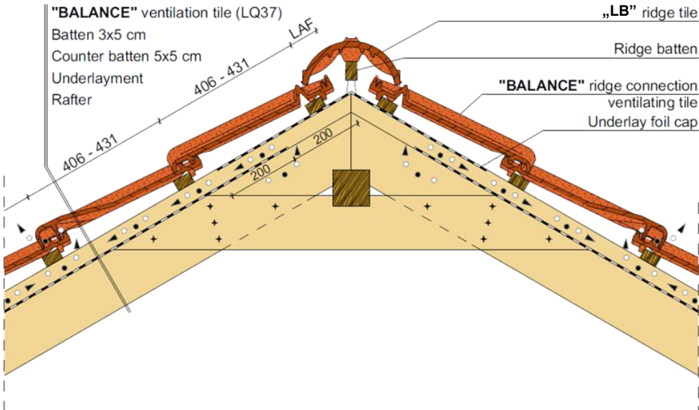
Ridge detail, with ventilation tile
