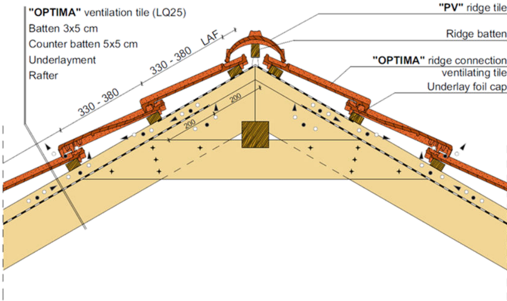
Ridge detail, with ventilation tile
