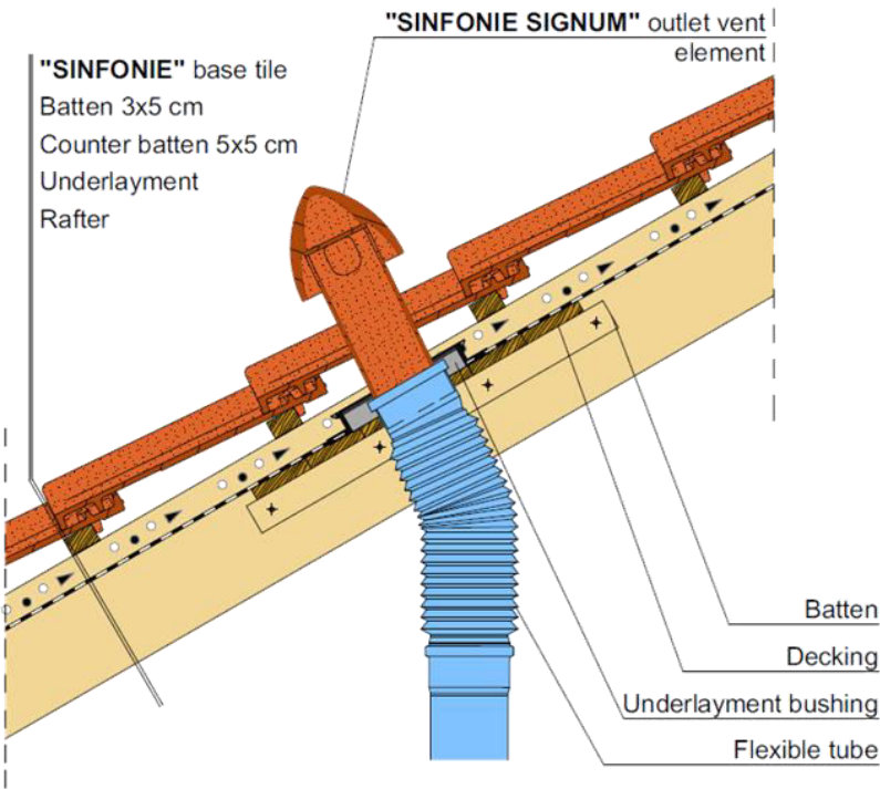
Clay ventilation outlet tile
