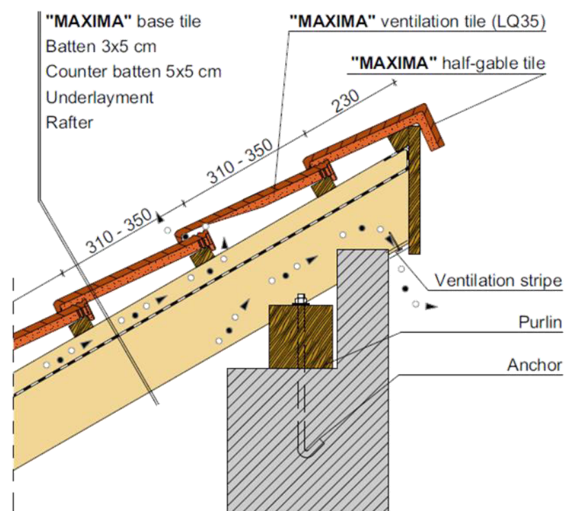
Shed ridge detail, with shad roof tile
