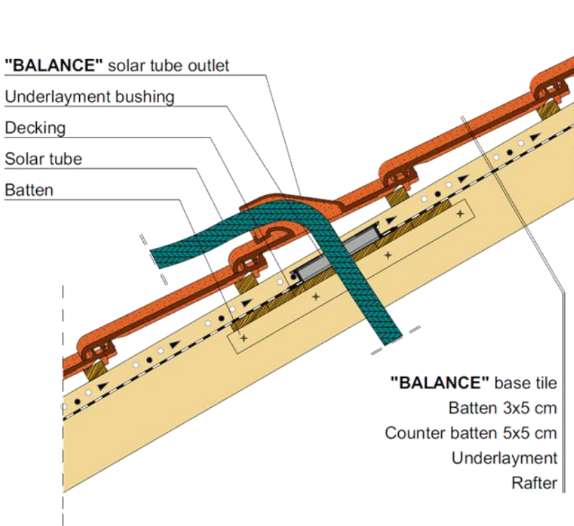
Clay solar tube outlet detail
