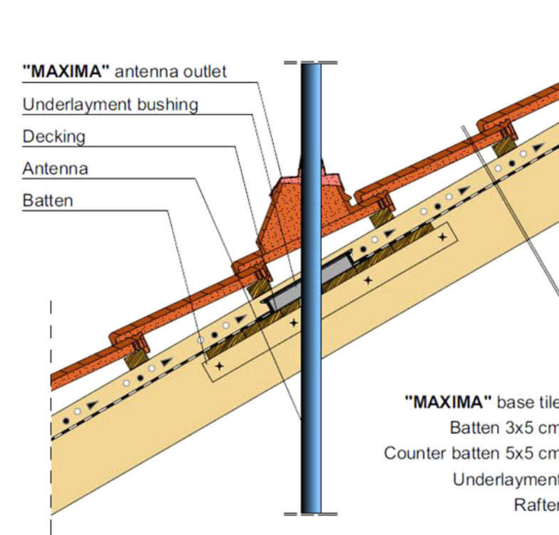
Clay antenna outlet tile
