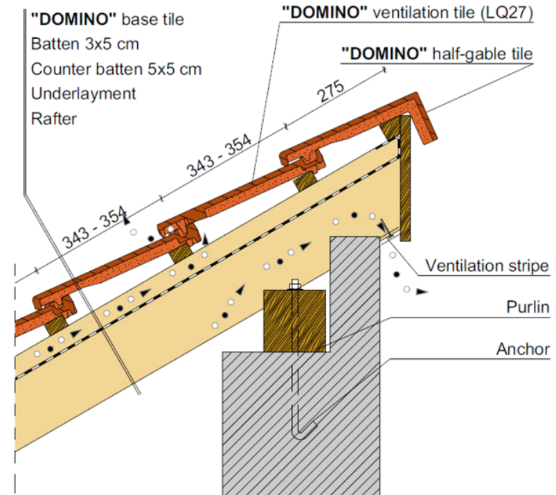
Shed ridge detail, with shad roof tile
