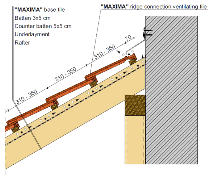
Wall connection detail
