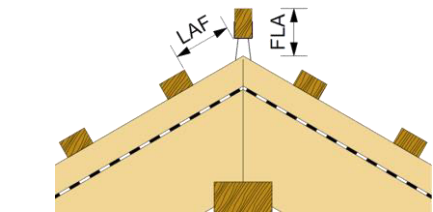
LAF: distance of the upper batten
