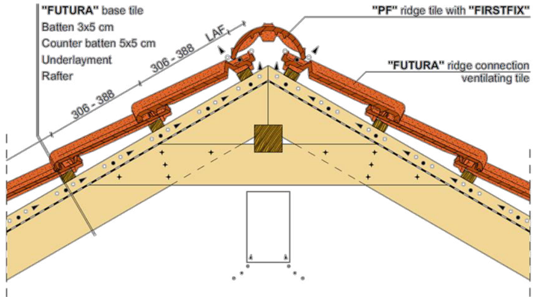
Ridge detail, with ridge connection ventilation tile
