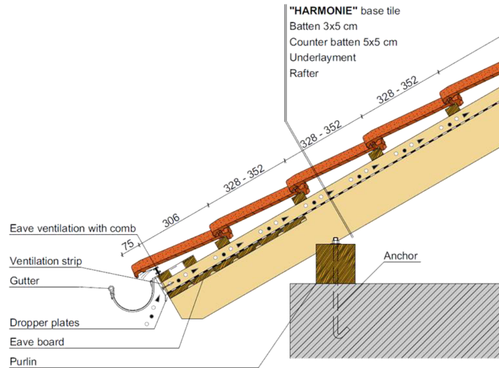
Eave detail
