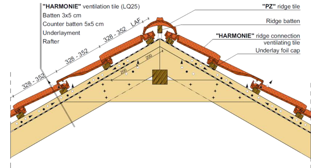
Ridge detail, with ventilation tile
