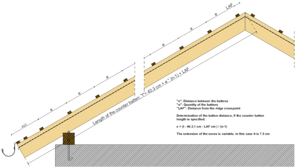
Roof batten alignment for "TITANIA" clay roof tile
