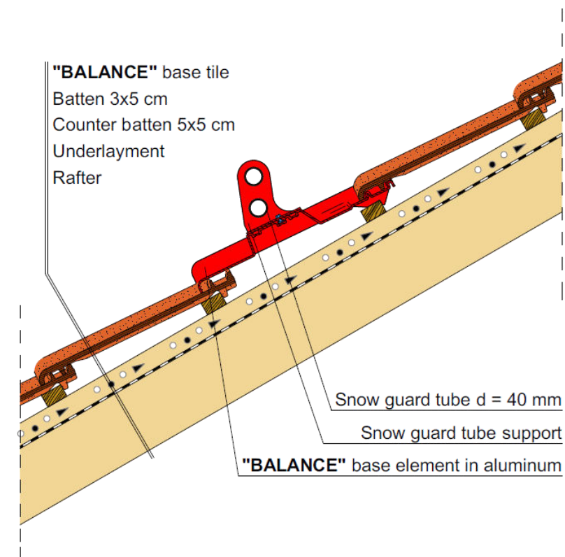
Snow guard tube placement
