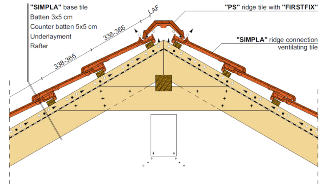
Ridge detail, with ridge connection ventilation tile
