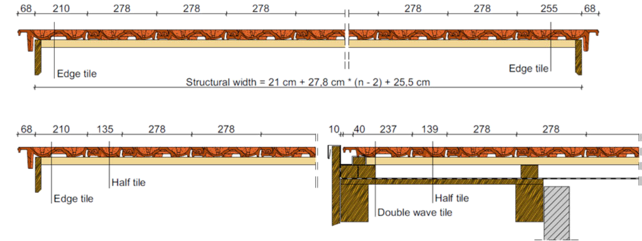
Structural width between the verge boards
