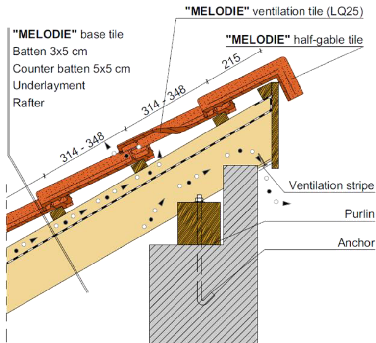
Shed ridge detail, with shad roof tile
