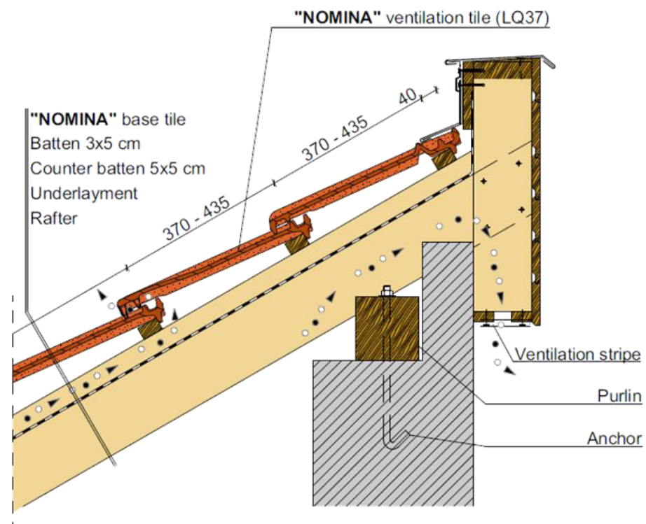
Shed ridge detail, with shad roof tile
