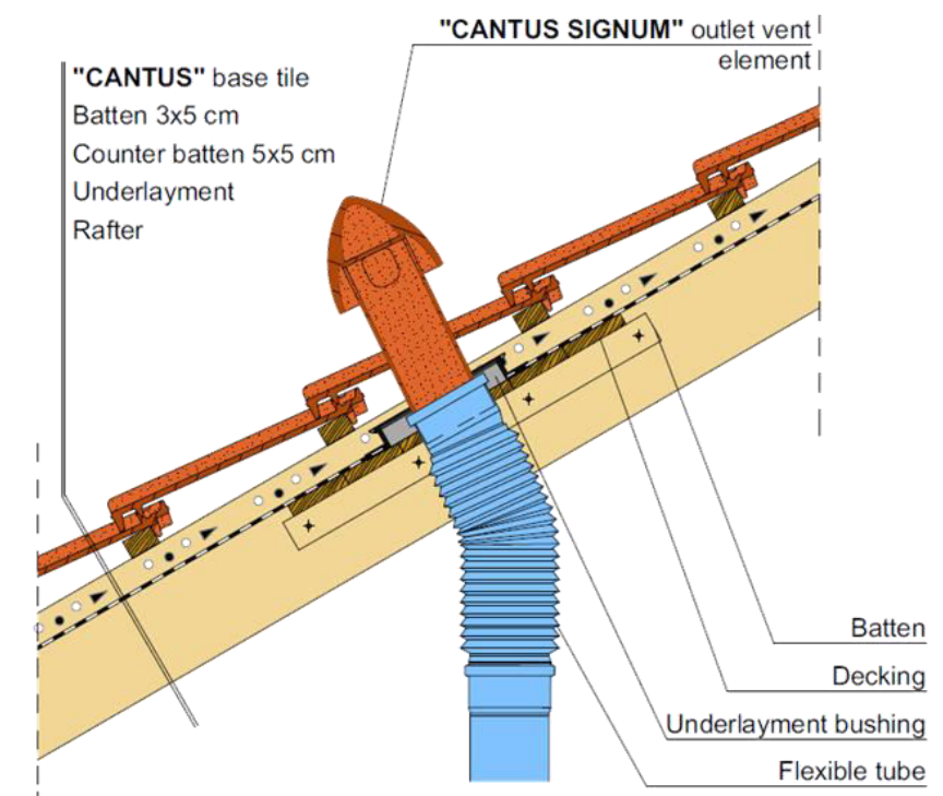
Clay ventilation outlet tile
