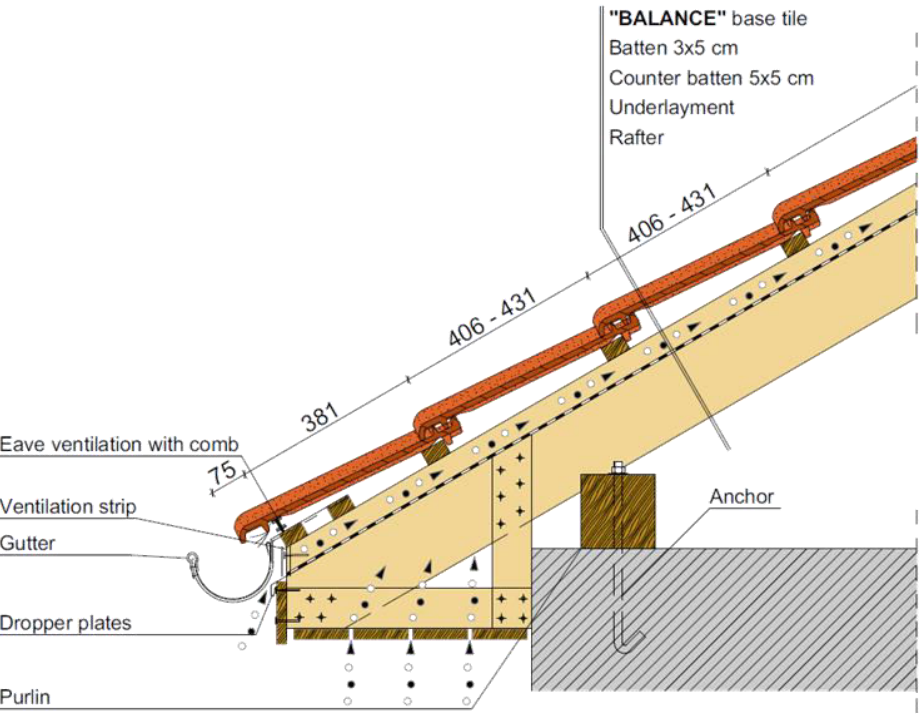
Closed eave detail
