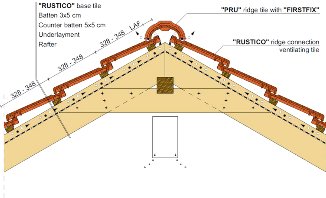
Ridge detail, with ridge connection ventilation tile
