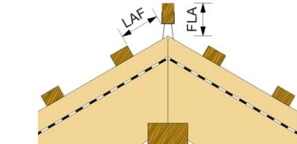
LAF: distance of the upper batten FLA: height of the ridge batten
