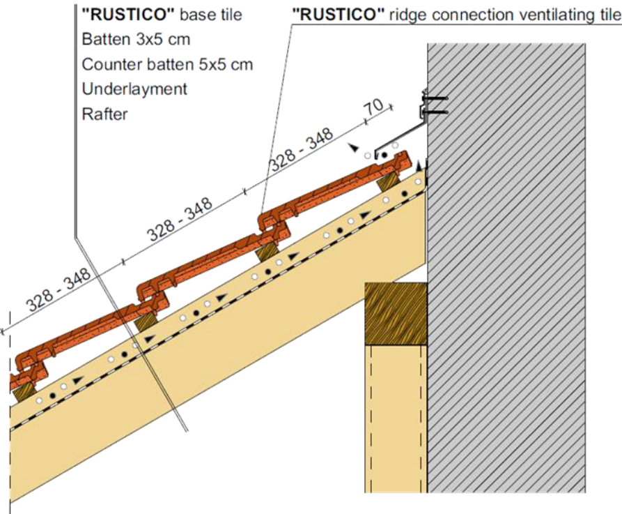
Wall connection detail
