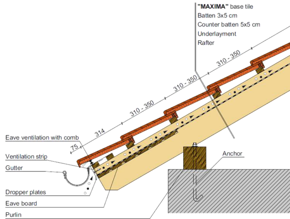
Eave detail
