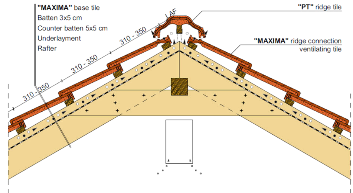
Ridge detail, with ridge connection ventilation tile
