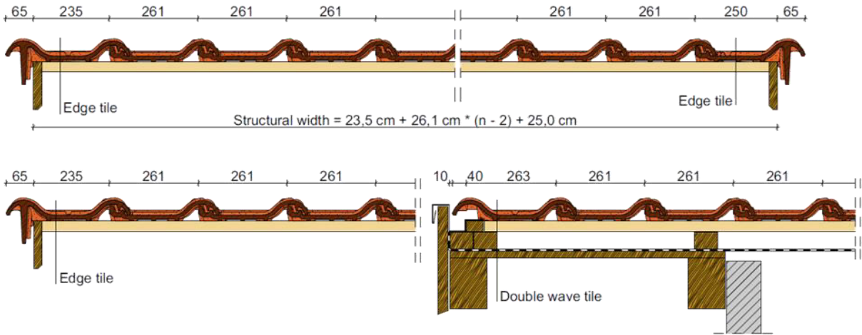
Structural width between the verge boards
