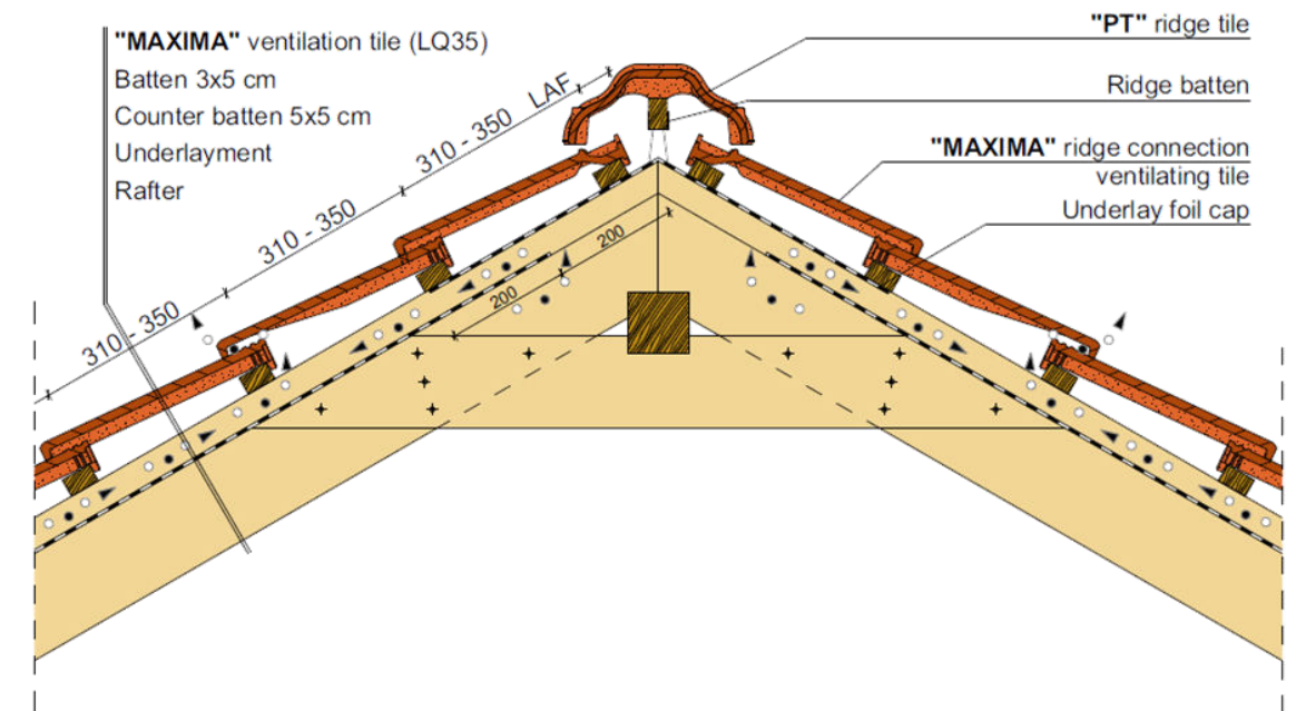
Ridge detail, with ventilation tile
