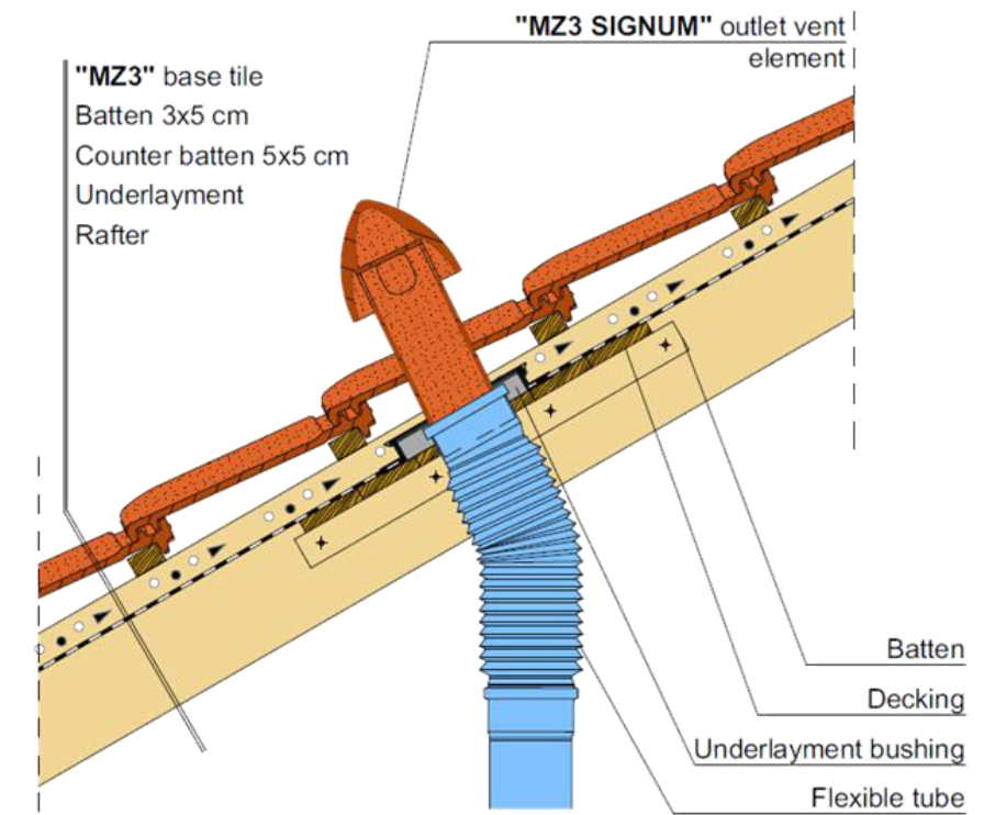
Clay ventilation outlet tile
