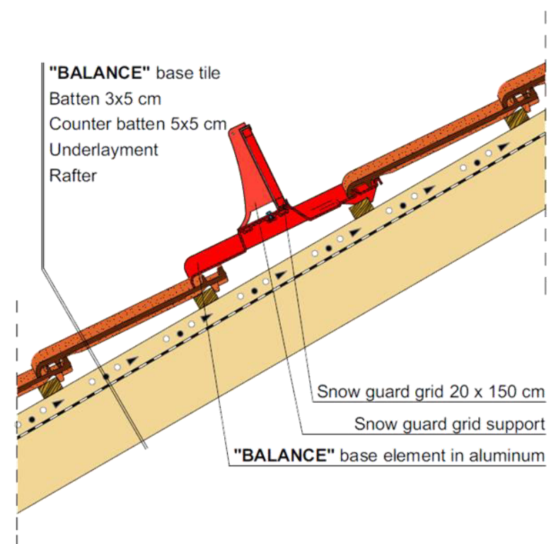
Snow guard grid placement
