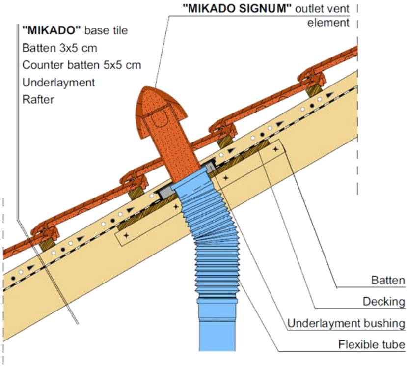
Clay ventilation outlet tile
