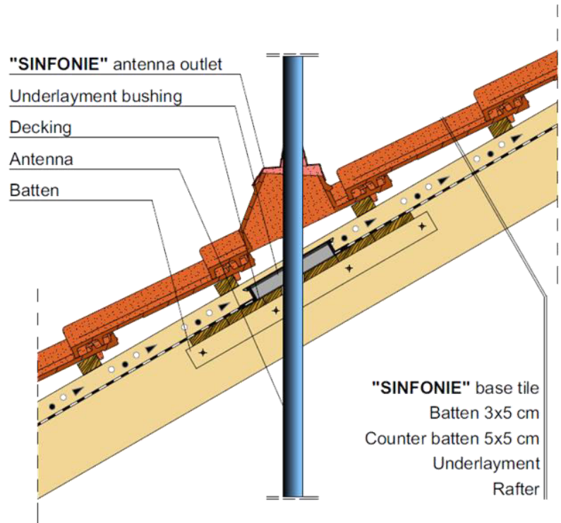
Clay antenna outlet tile
