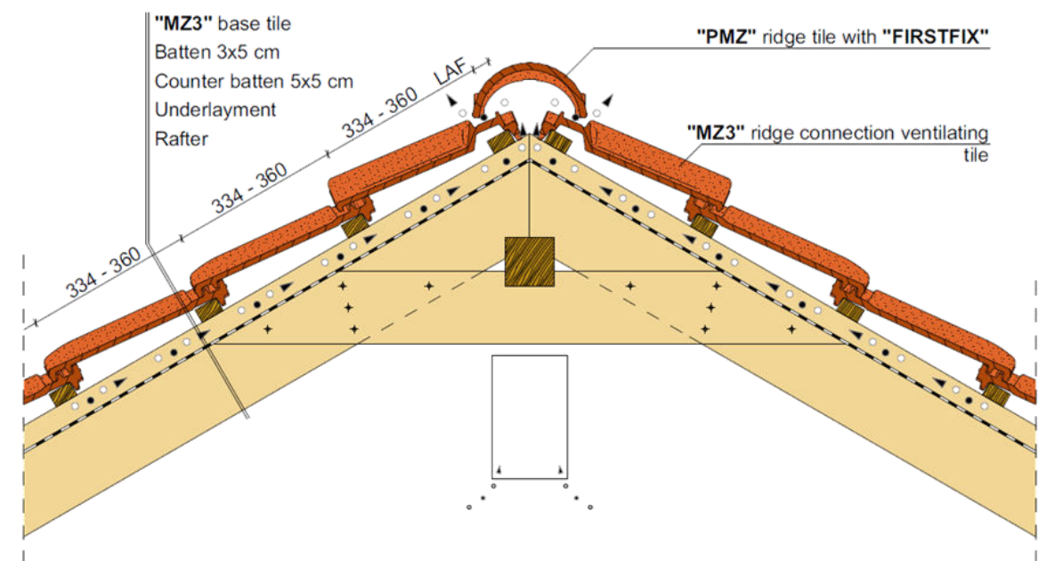
Ridge detail, with ridge connection ventilation tile
