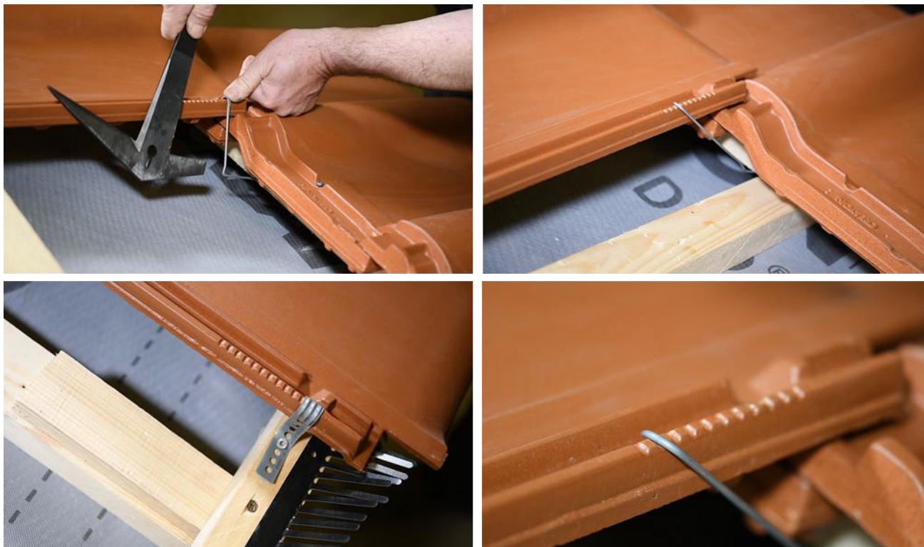
Nail-in, mount-on and the universal stormclip installation, and the grooves in the side lock where the mount-on stormclip can be hooked
