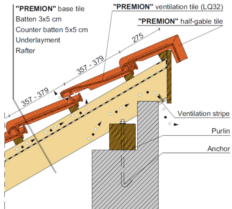
Shed ridge detail, with shad roof tile
