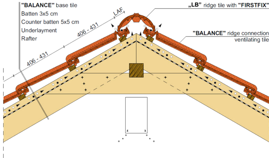
Ridge detail, with ridge connection ventilation tile
