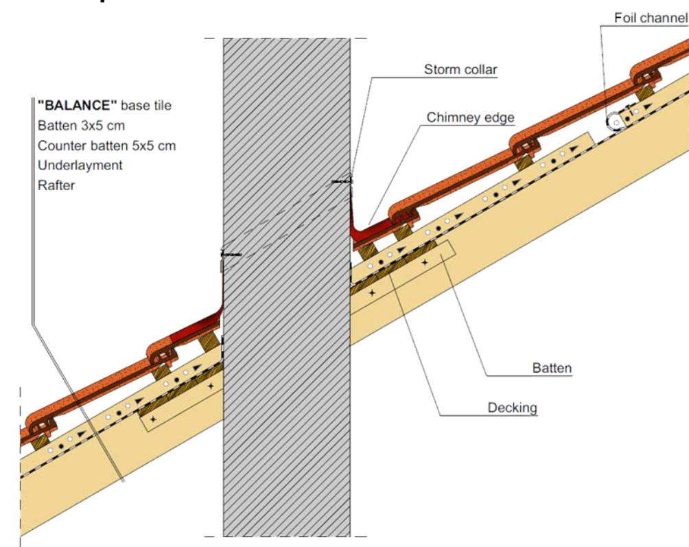
Chimney connection detail
