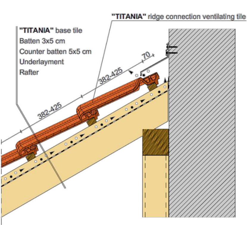
Wall connection detail
