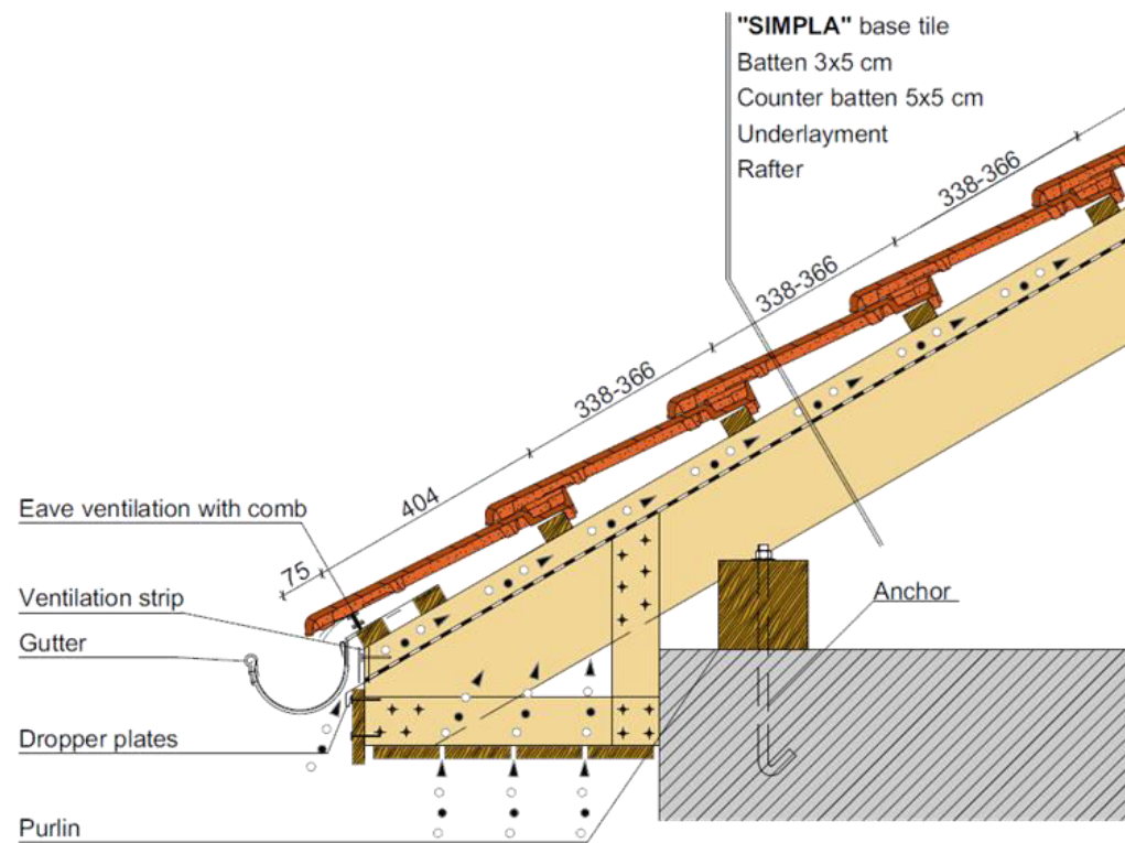
Closed eave detail
