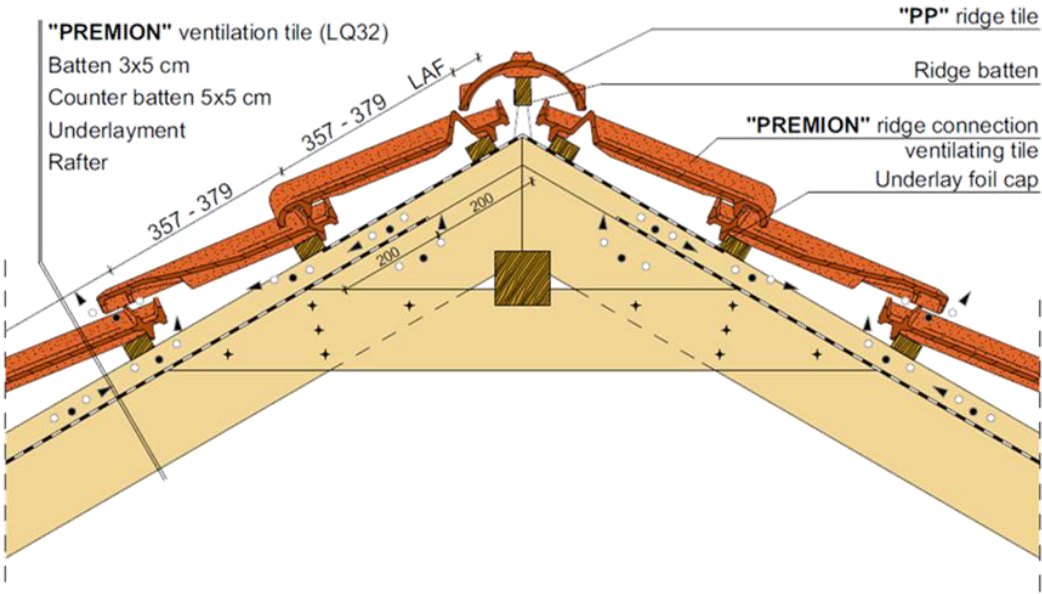
Ridge detail, with ventilation tile
